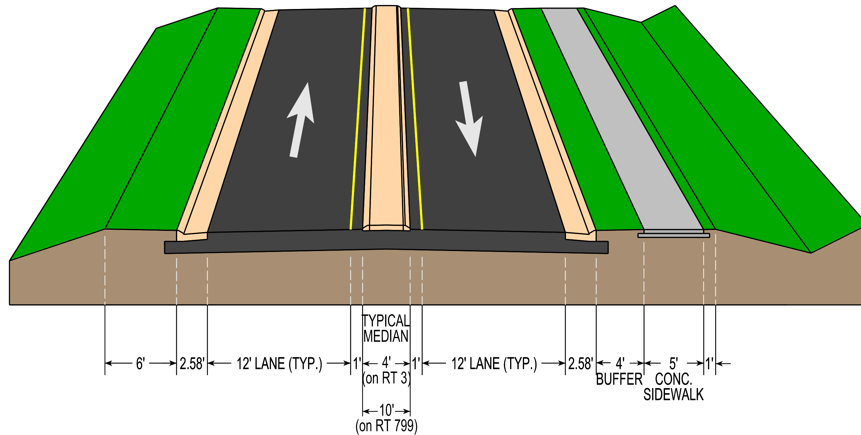
Route 3 WB & McDevitt SB Roundabout Approach
