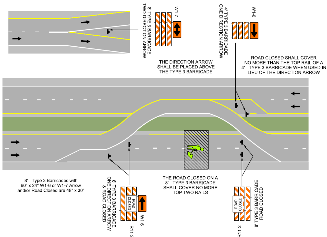
Figure 6F-9, Type 3 Barricade Placement Guidelines 2 See Figures TTC-43 and TTC-44 for installation details
