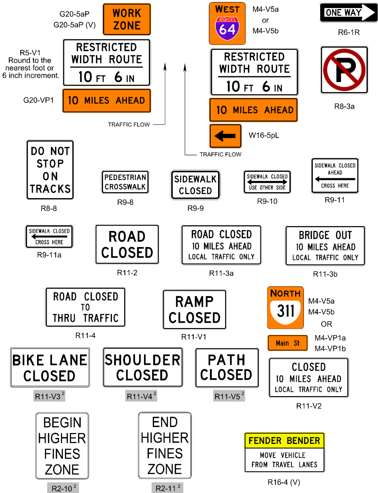
Figure 6F-2, Regulatory Signs and Plaques in Temporary Traffic Control (Sheet 2 of 2) 2
