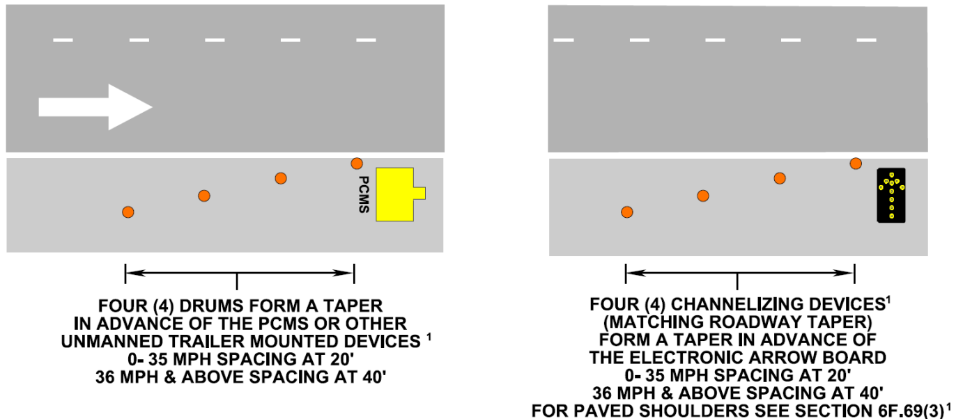
Figure 6F-6, Channelizing Devices for PCMS, Arrow Board and other Trailer Mounted Devices 1
