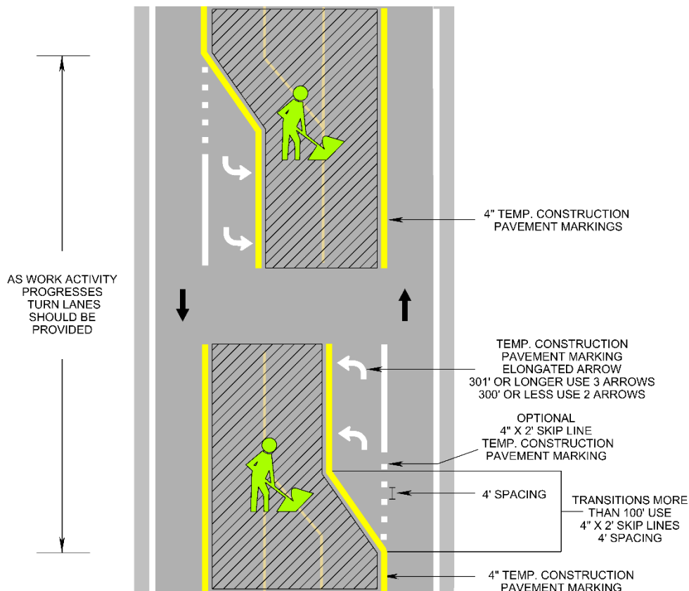
Figure 6F-10, Temp. 2 Construction Pavement Marking for Tapers and Turn Lanes
