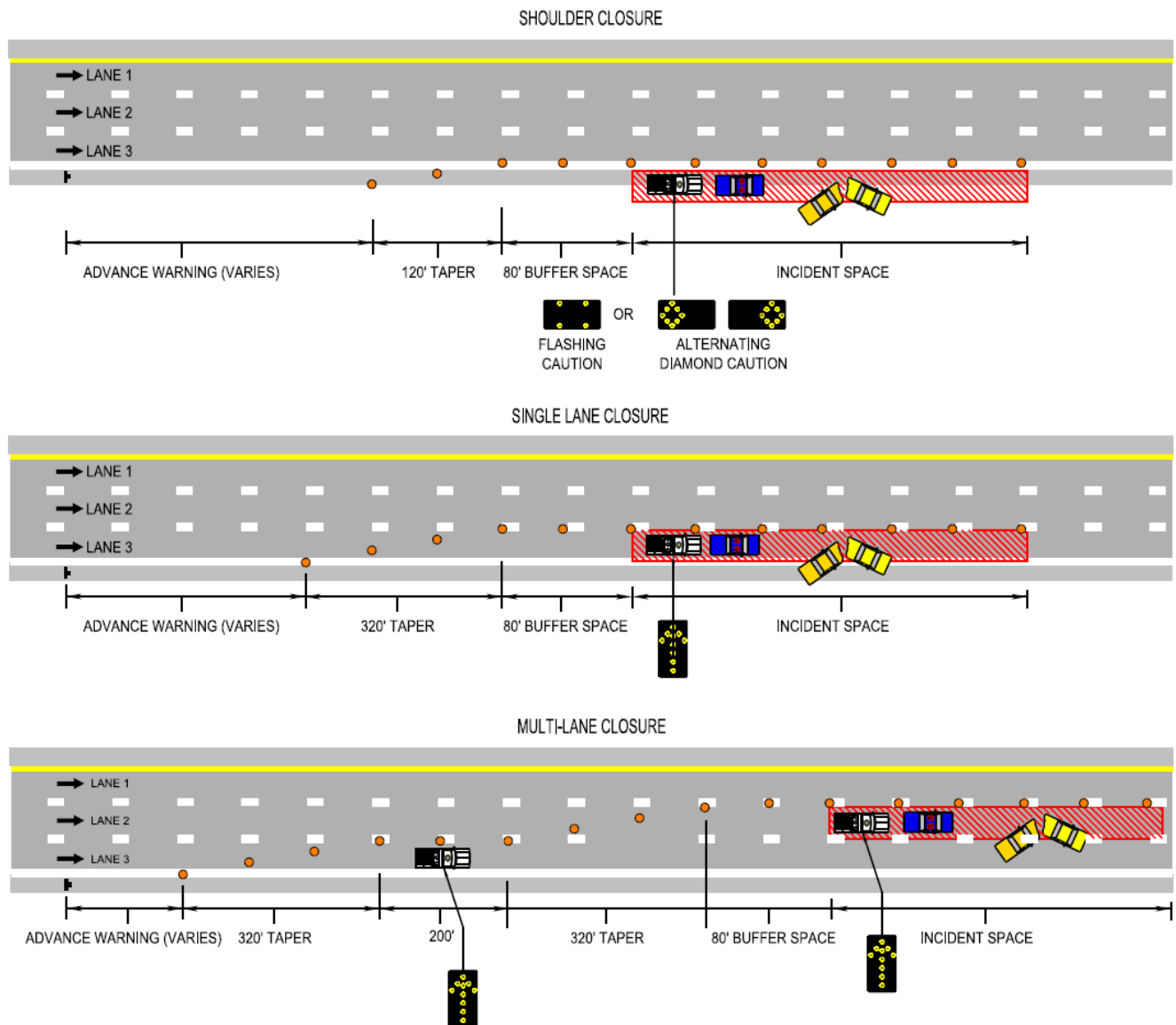
Figure 6I-1, Desired Initial Incident Scene Setups and Identification by Travel Lane Numbering 2
