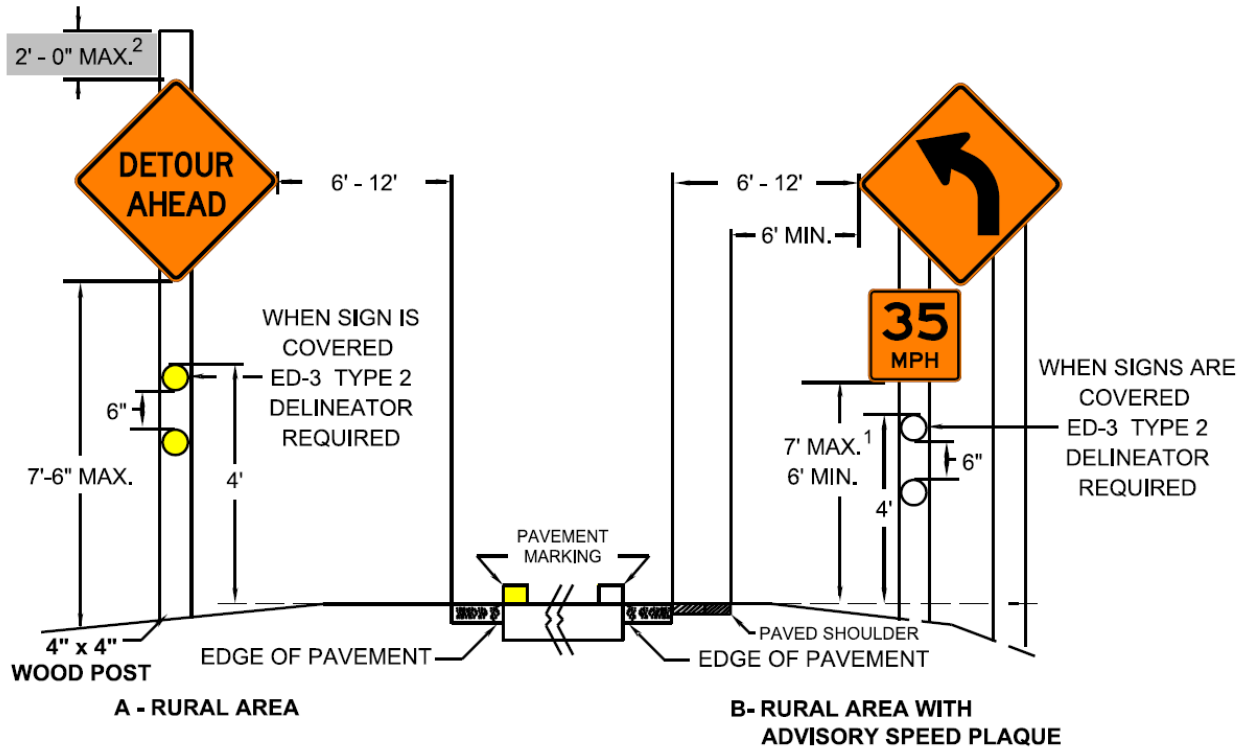
Figure 6F-1, Height and Lateral Location of Signs – Typical Post-Mounted Installations 2
