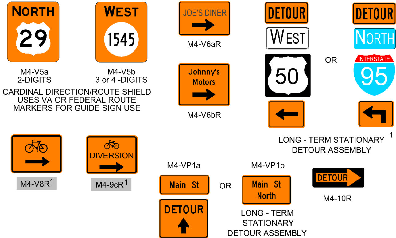
Figure 6F-5, Exit, Pull Off Area, Exit Open, and Detour Signs for Temporary Traffic Control
