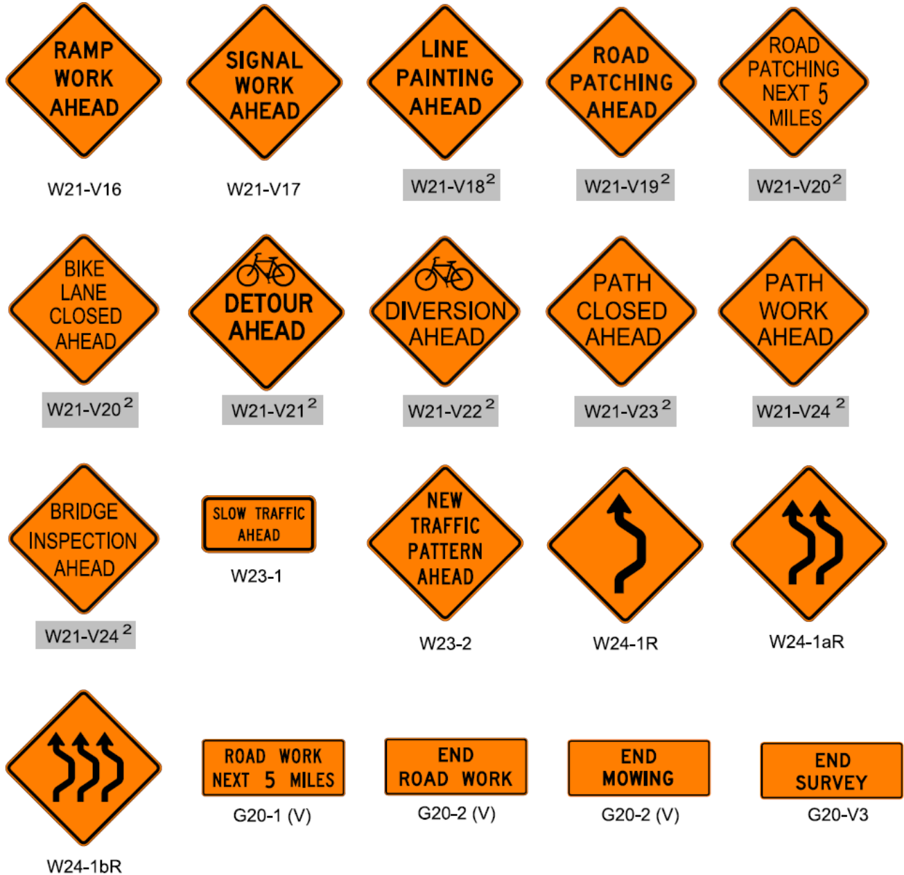
Figure 6F-3, Warning Signs and Plaques in Temporary Traffic Control (Sheet 5 of 5) 1
