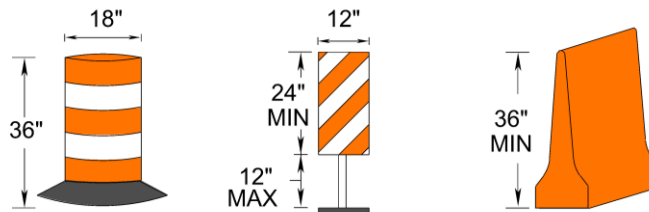
GROUP 2 DRUM, VERTICAL PANEL, & LONGITUDINAL CHANNELIZING DEVICE
