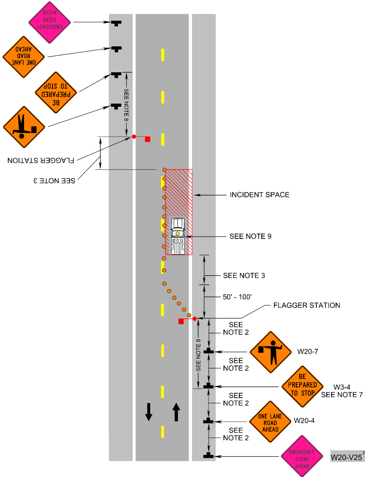
Incident Blocking a Lane on a Two-Lane Roadway (Figure TIMC-5.2)
