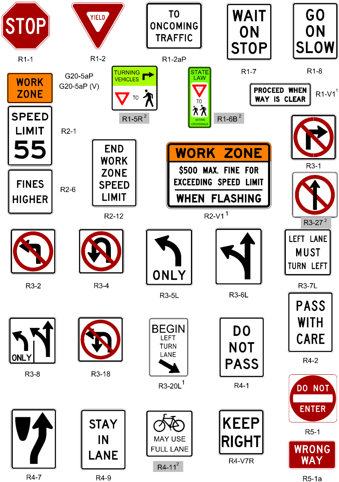
Figure 6F-2, Regulatory Signs and Plaques in Temporary Traffic Control (Sheet 1 of 2) 2
