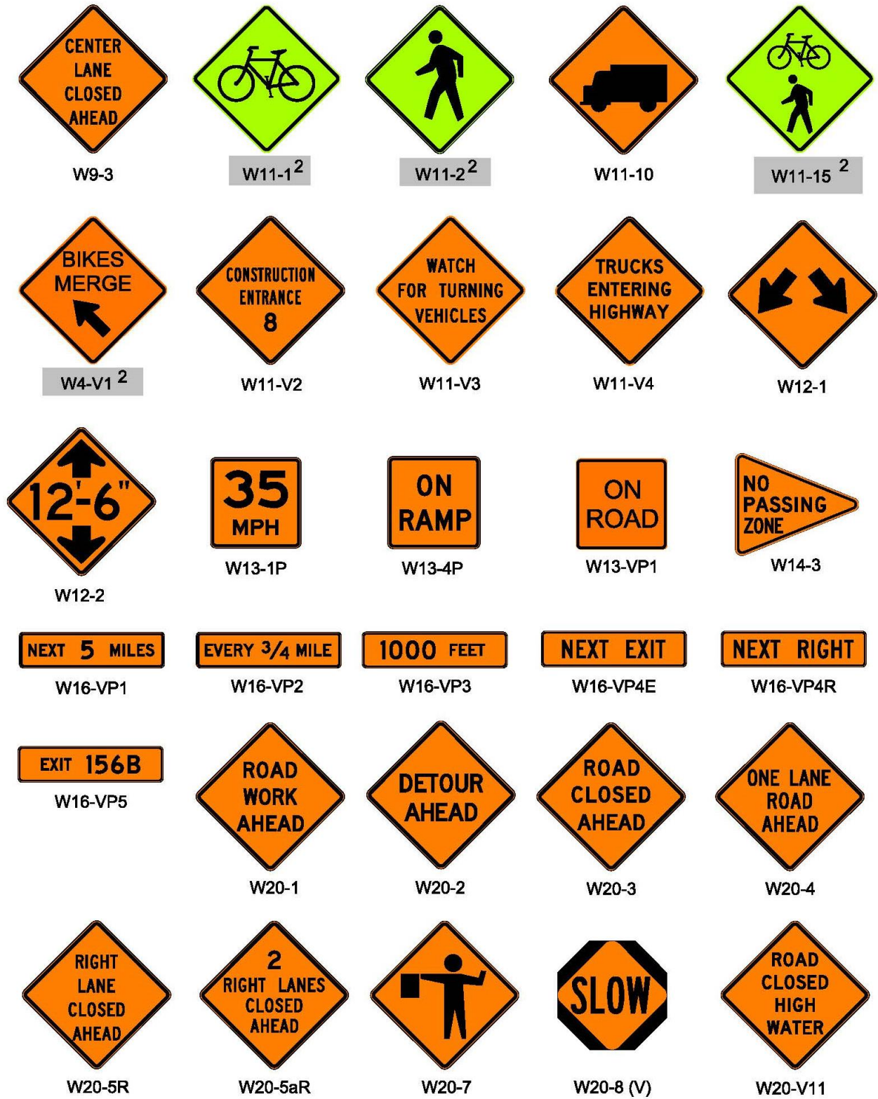
Figure 6F-3, Warning Signs and Plaques in Temporary Traffic Control (Sheet 3 of 5) 2,1
