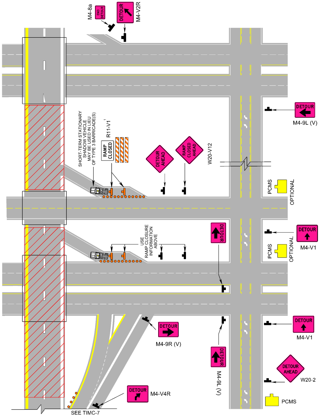
Highway Closure Incident with a Temporary Detour (Figure TIMC-8.1)
