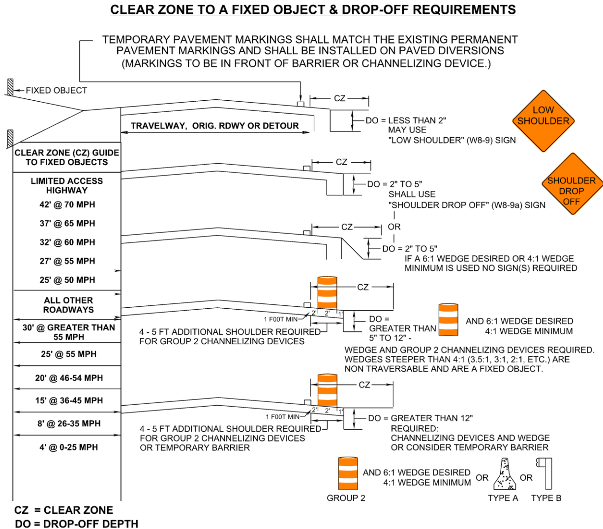
Figure 2, Clear Zone and Drop-Off Requirements
