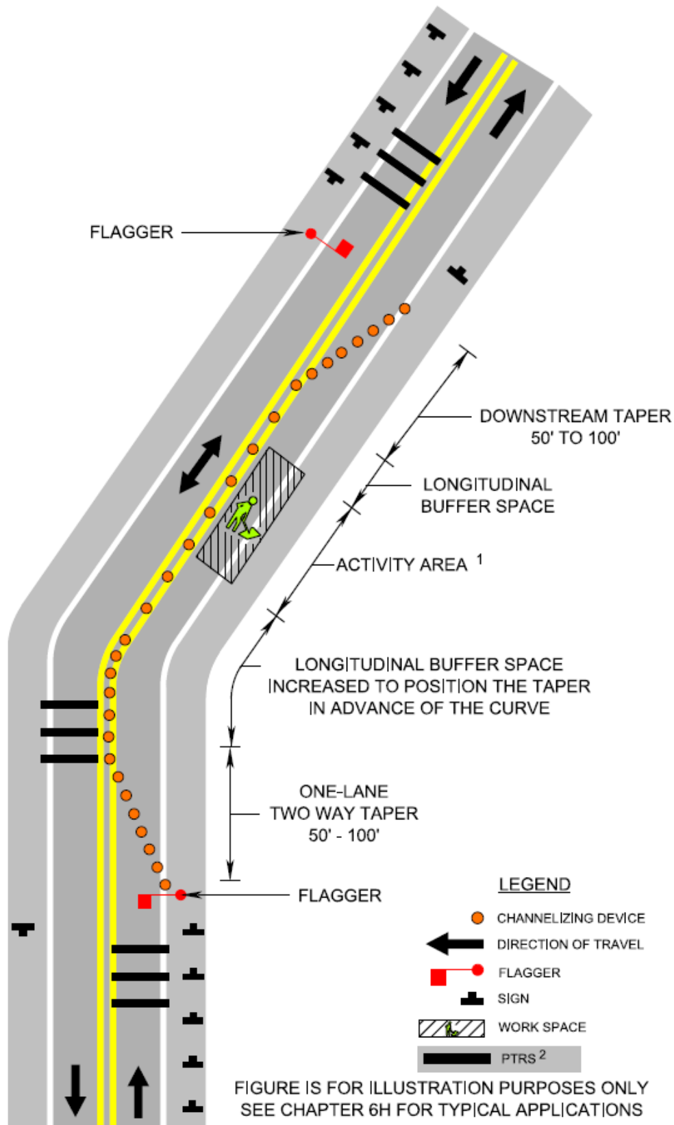
Figure 6C-3, Example of a One-Lane, Two-Way Taper 2
