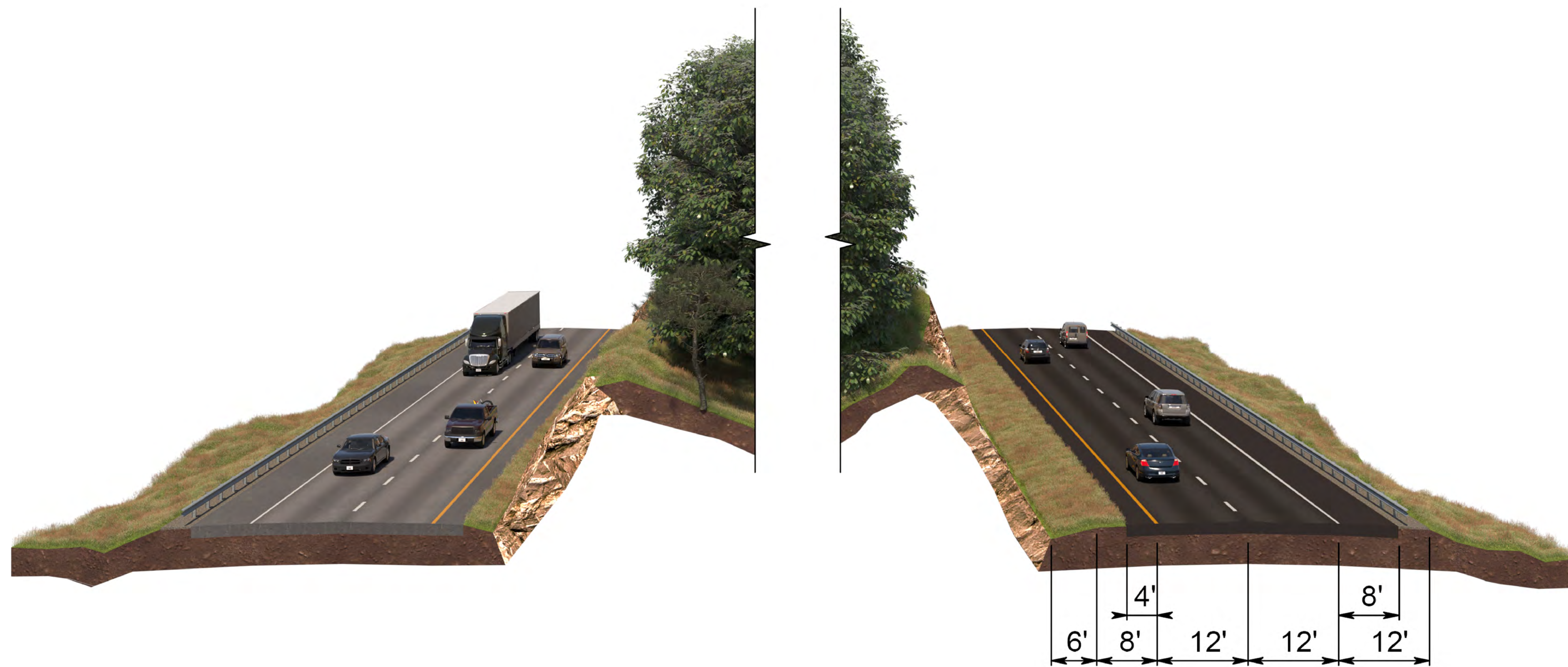
WESTBOUND (EXISTING ROUTE 58 - WIDTHS VARY)
